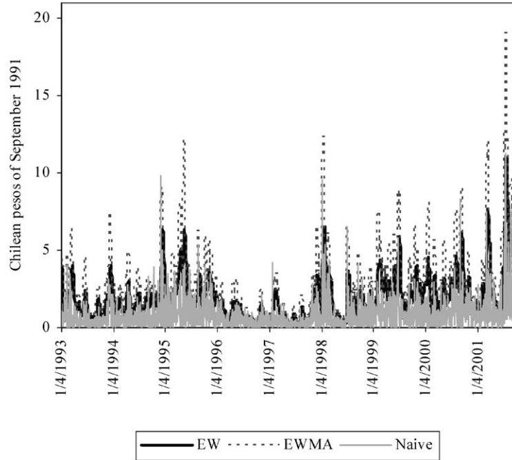
Fig. 8. Estimates of Chile's nominal exchange rate volatility: January 1993–September 2001. Source: Based upon on daily data of the observed market exchange rate, provided by the Central Bank of Chile. The observed exchange rate series was deflated by the daily percent variation of the Unidad de Fomento (base = 1, September 1, 1991). EW stands for exponentially weighted and EWMA for exponentially weighted moving average.
