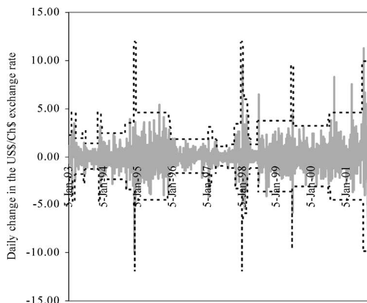
Fig. 9. Daily changes of Chile's US$/Ch$ exchange rate: January 1993–September 2001. Source: Author's elaboration. The US$/Ch$ rate was previously deflated by the UF. Change points were estimated by the ICSS algorithm; the dotted lines represent \pm 3 standard deviations.
